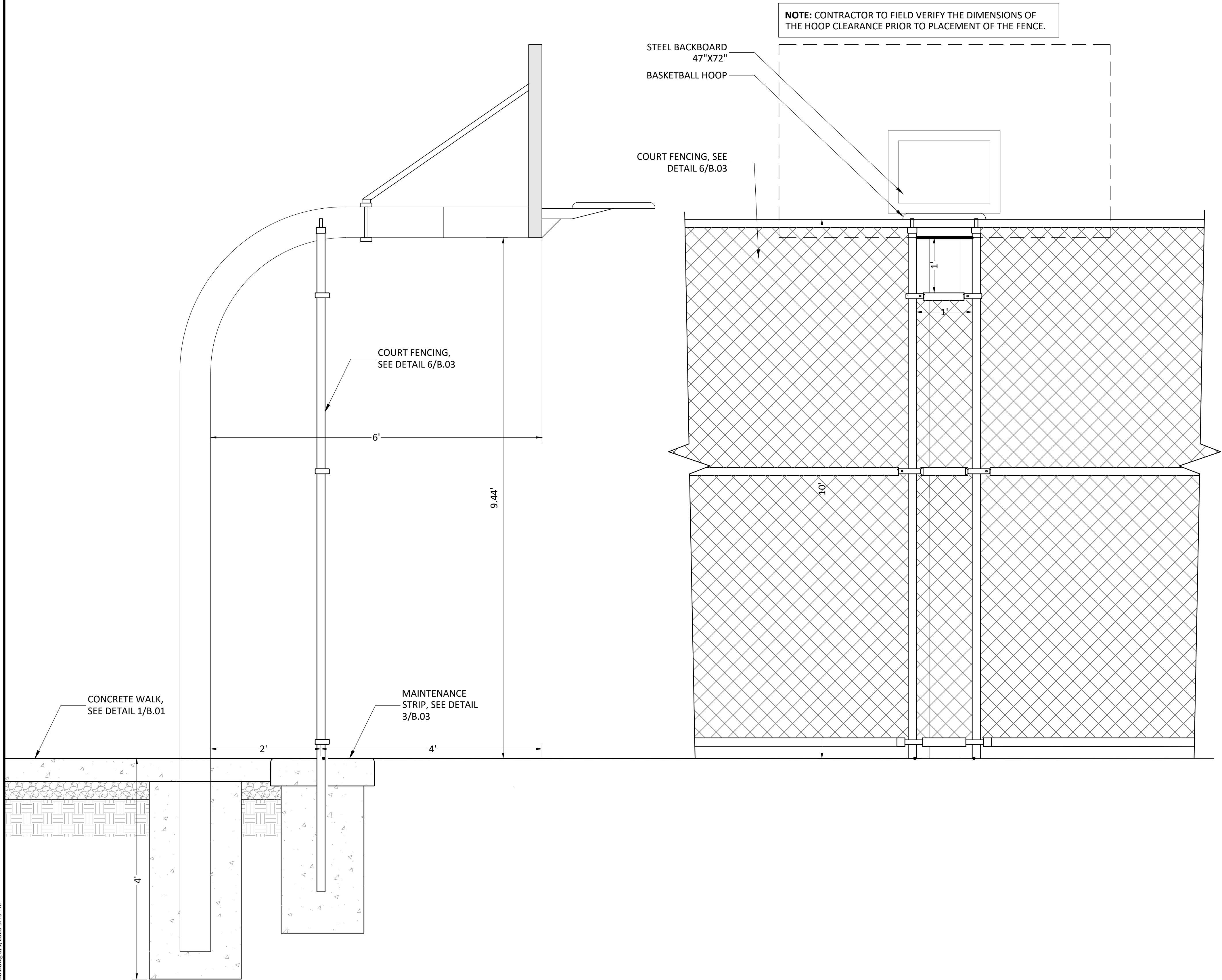
1 BASKETBALL HOOP LAYOUT
