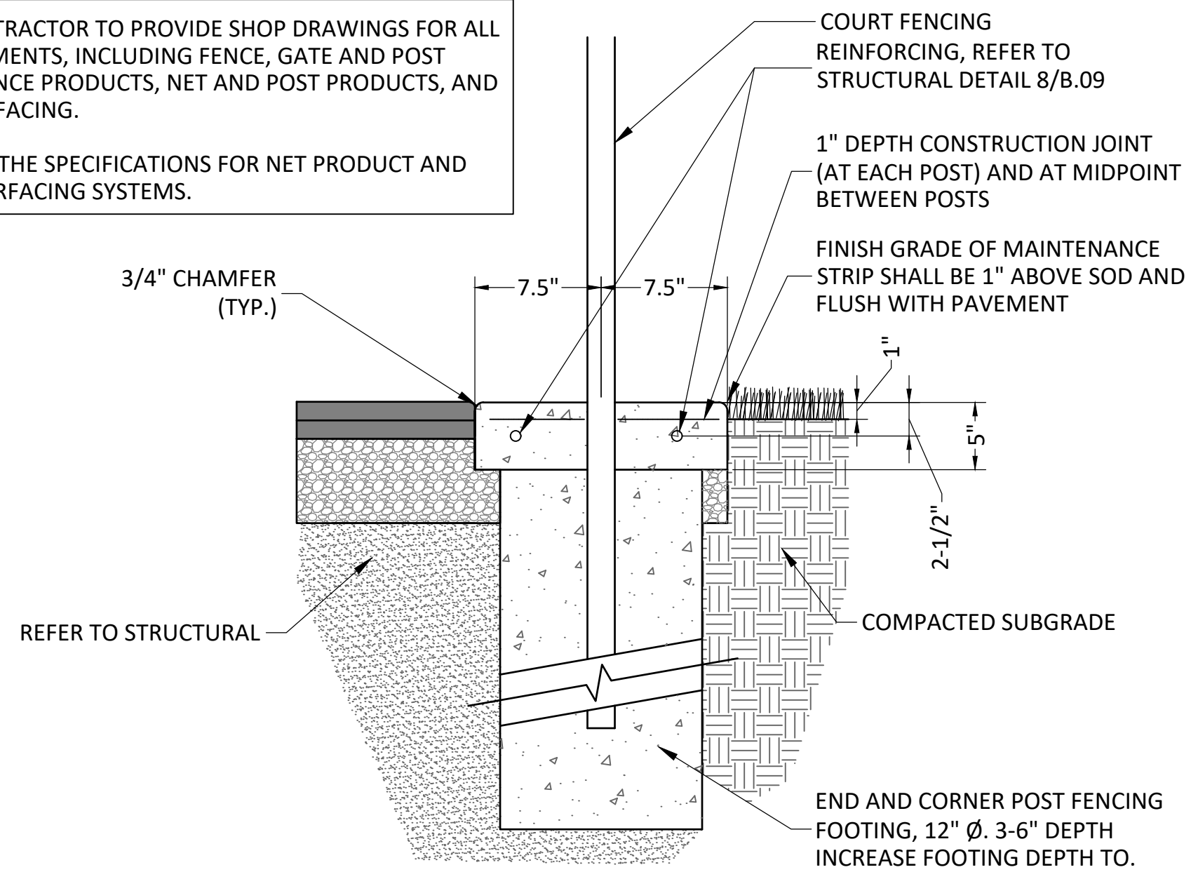
3 MAINTENANCE STRIP @ FENCE CONCRETE PIER
