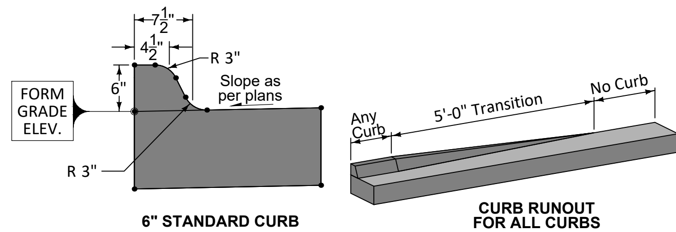
6" STANDARD CURB
