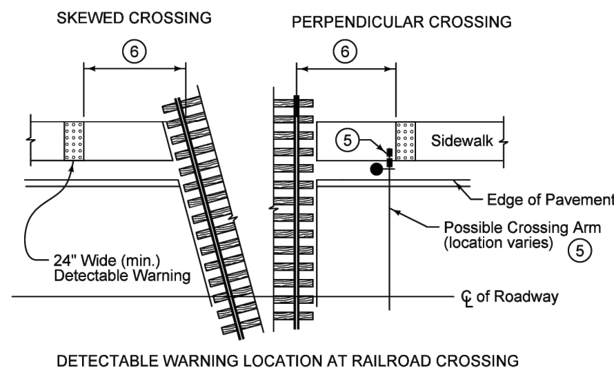
DETECTABLE WARNING LOCATION AT RAILROAD CROSSING
