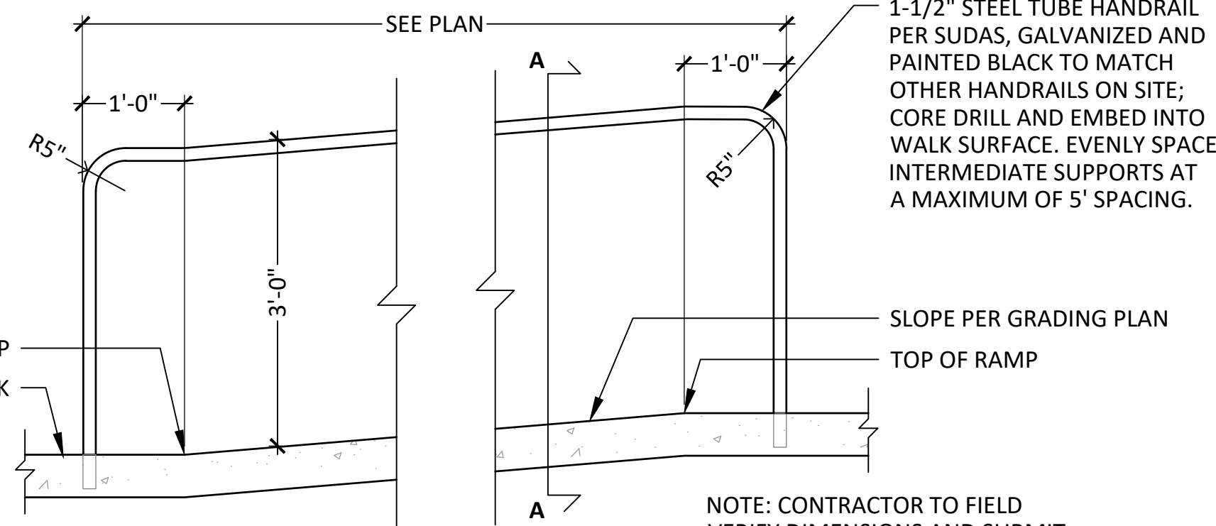
7 SECTION: RAMP WITH HANDRAIL SCALE: N.T.S.
