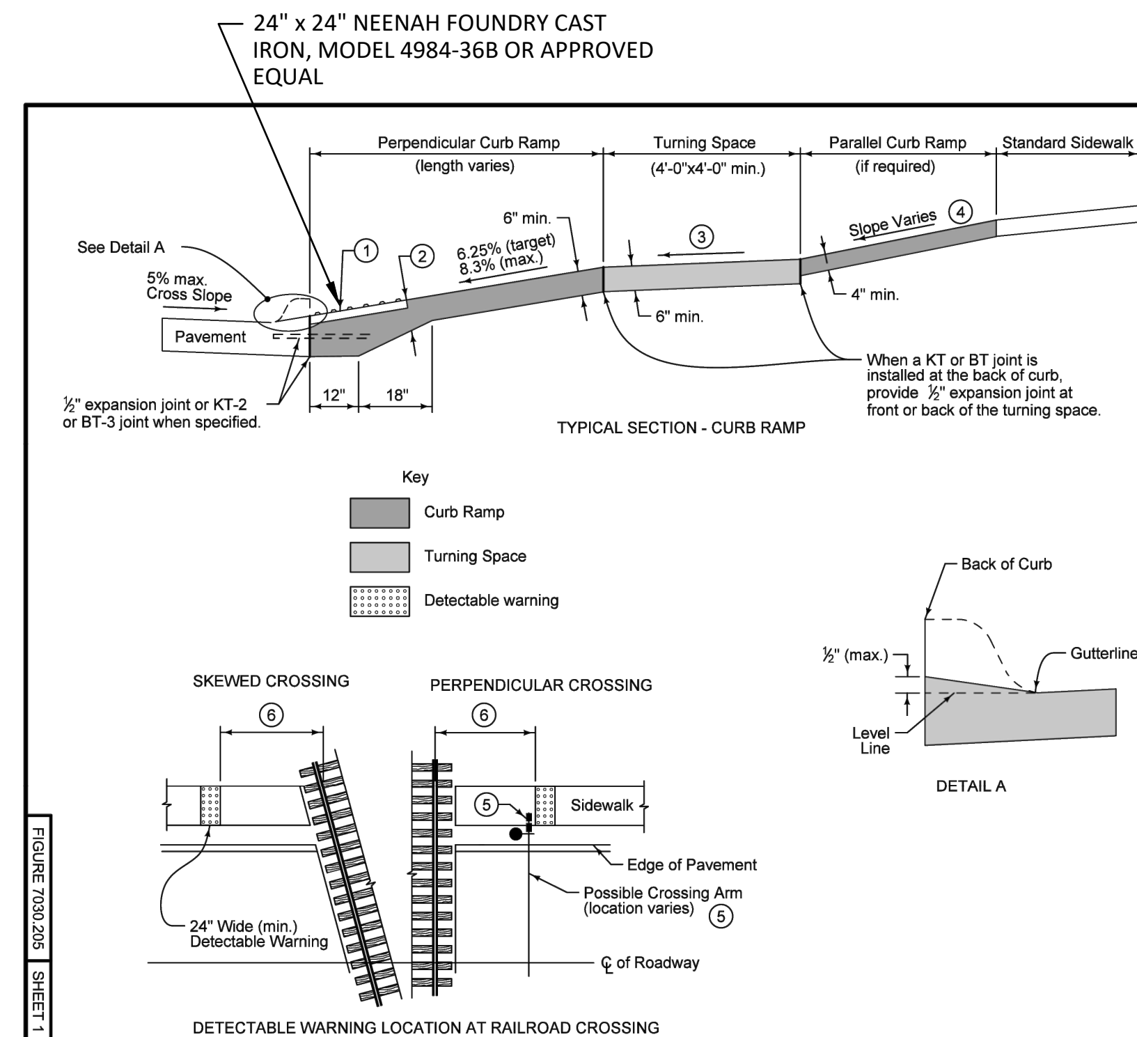
DETECTABLE WARNING LOCATION AT RAILROAD CROSSING
