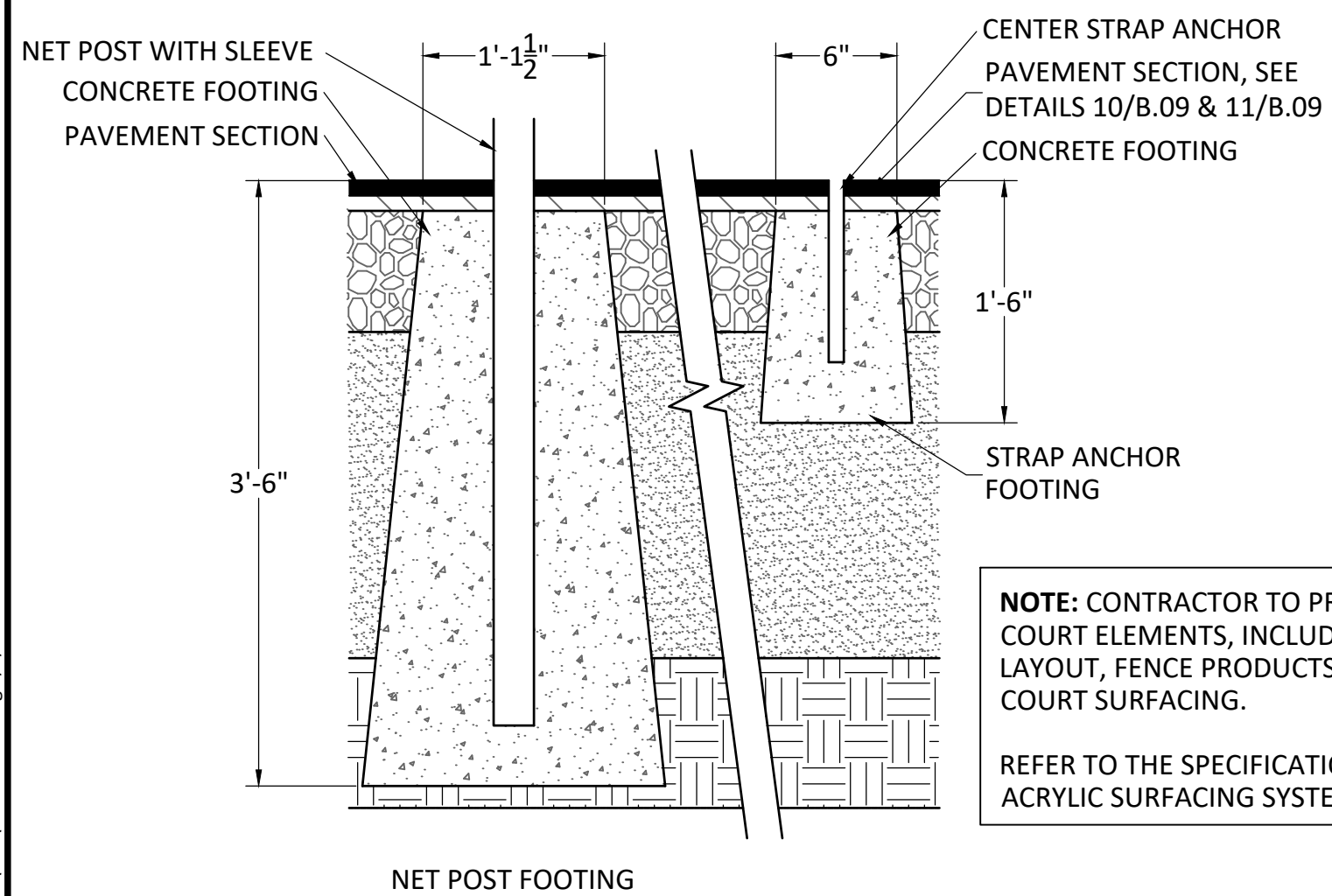
5 NET POST AND STRAP CONCRETE PIERS
